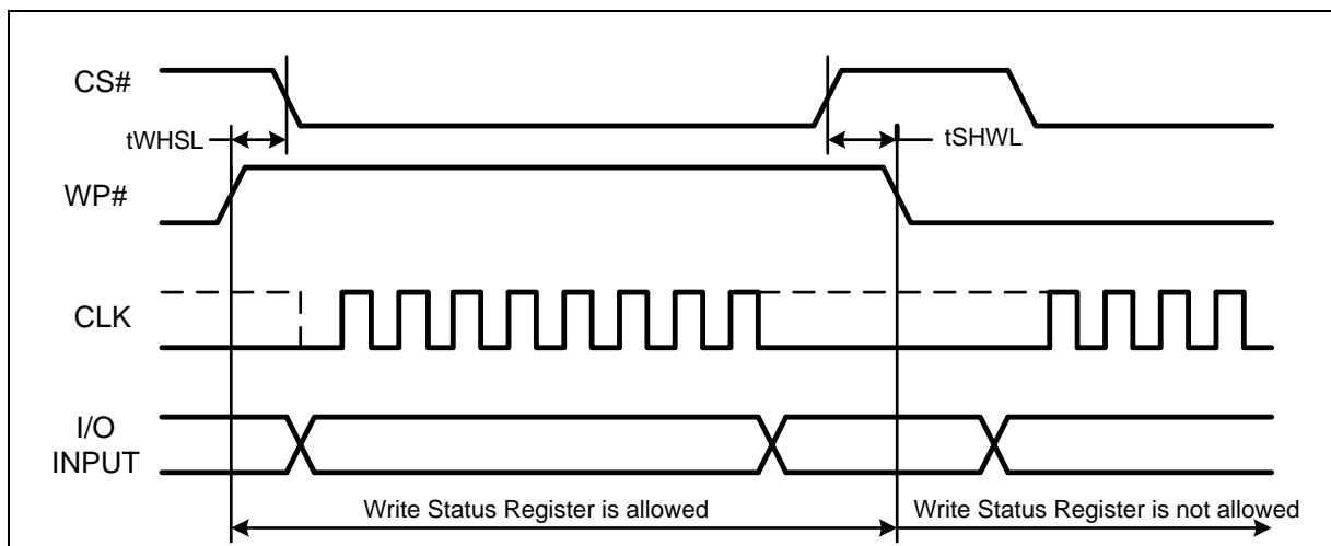
Figure 67 WP# Timing
