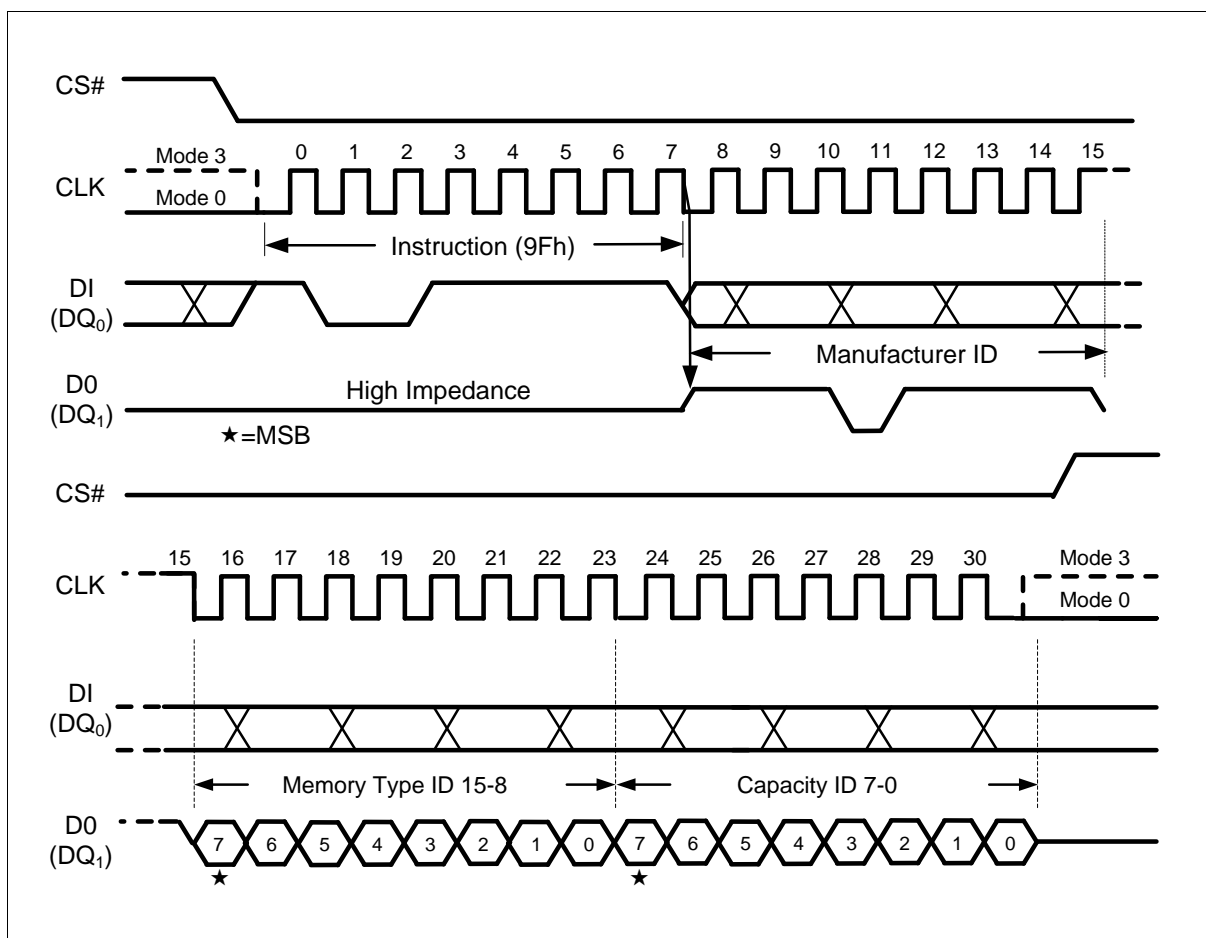
Figure 50 Read JEDEC ID Instruction (SPI Mode)
