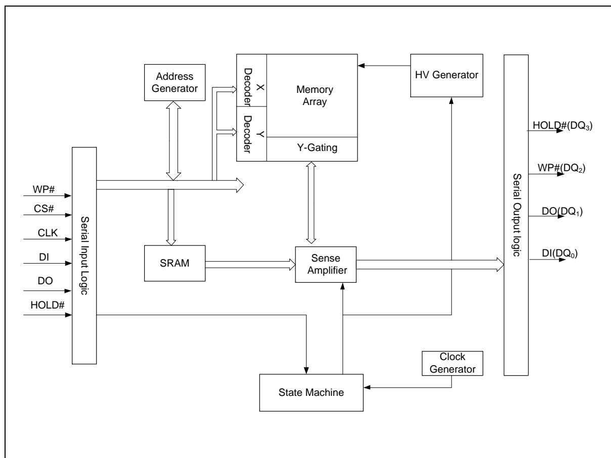
Figure 1 FM25W16 Serial Flash Memory Block Diagram
