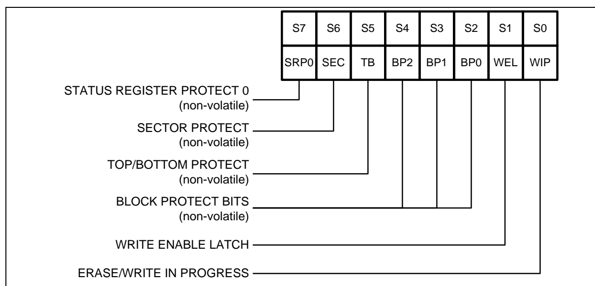
Figure 5 Status Register 1
