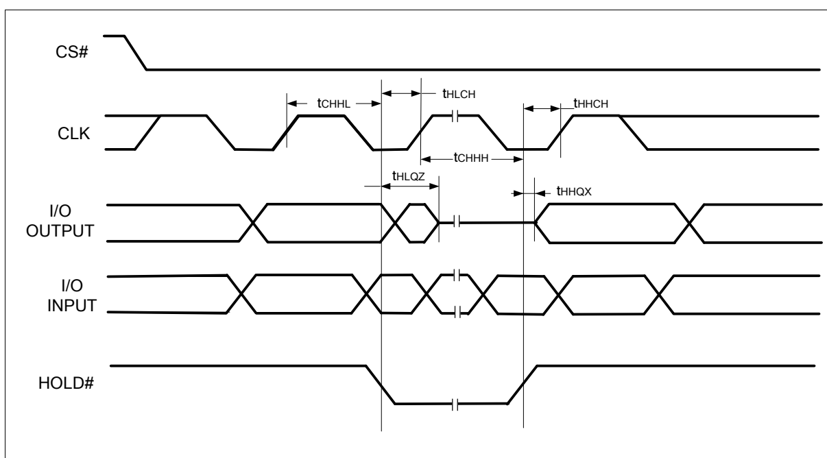
Figure 66 Hold Timing
