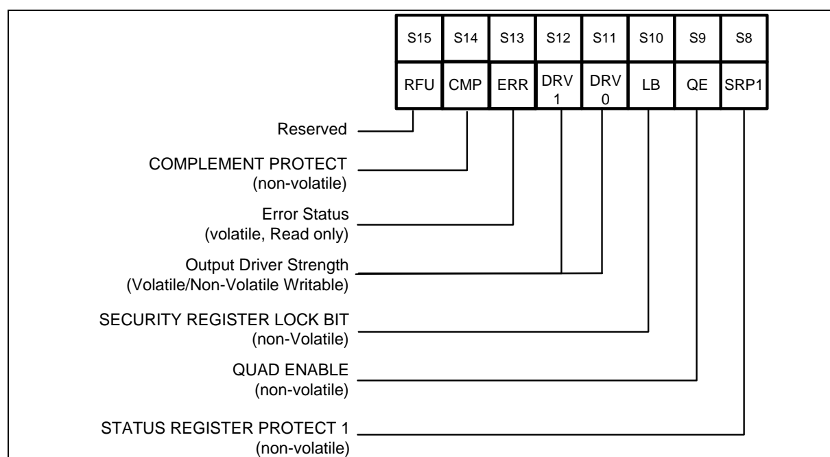
Figure 6 Status Register 2
