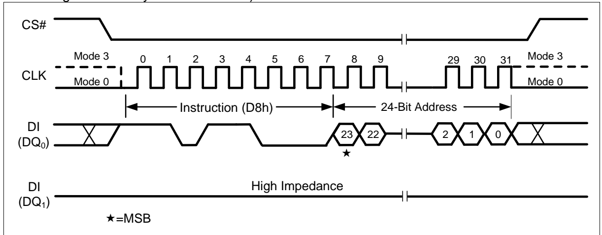
Figure 36 64KB Block Erase Instruction (SPI Mode)
