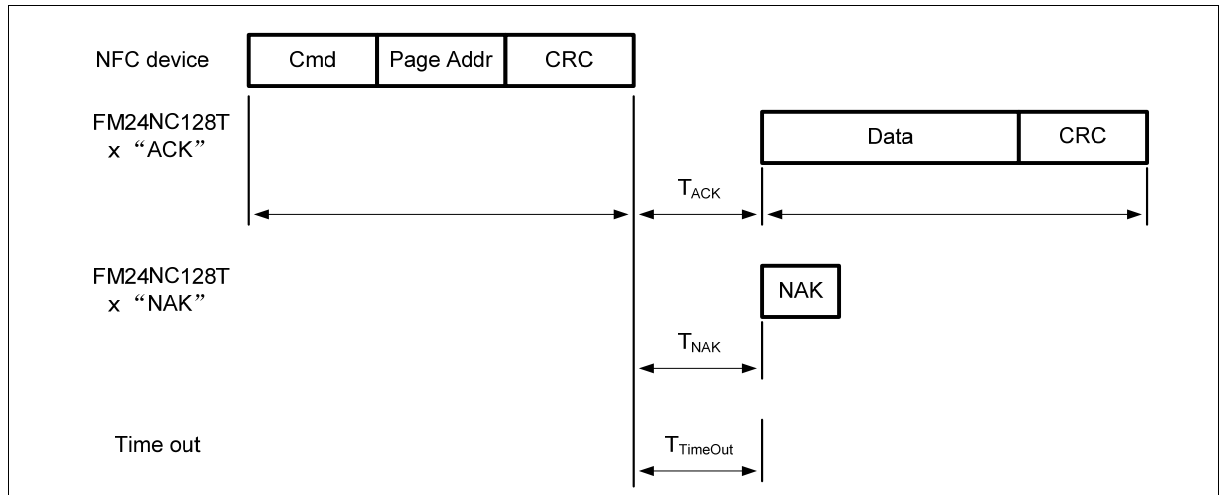
Figure 26 READ64B command
