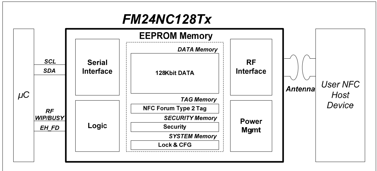
Figure 1 Block Diagram of FM24NC128Tx
