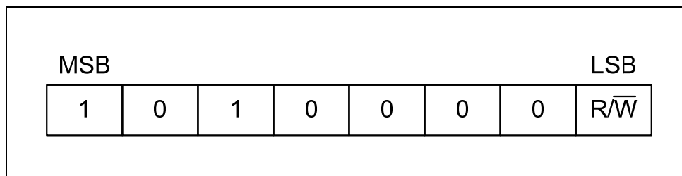
Figure 8 Device address of two wire serial interface
