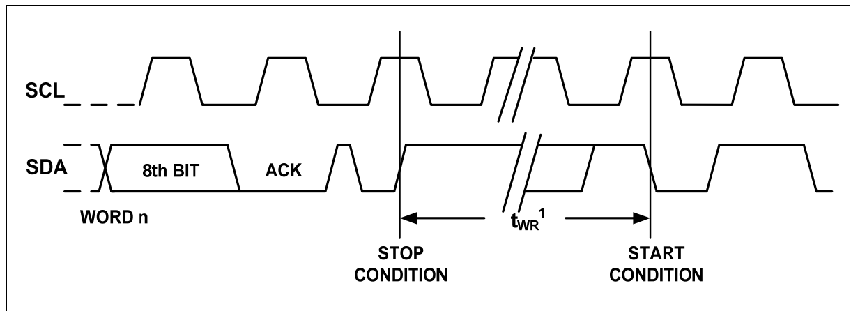
Figure 4 Writing Cycle Timing
