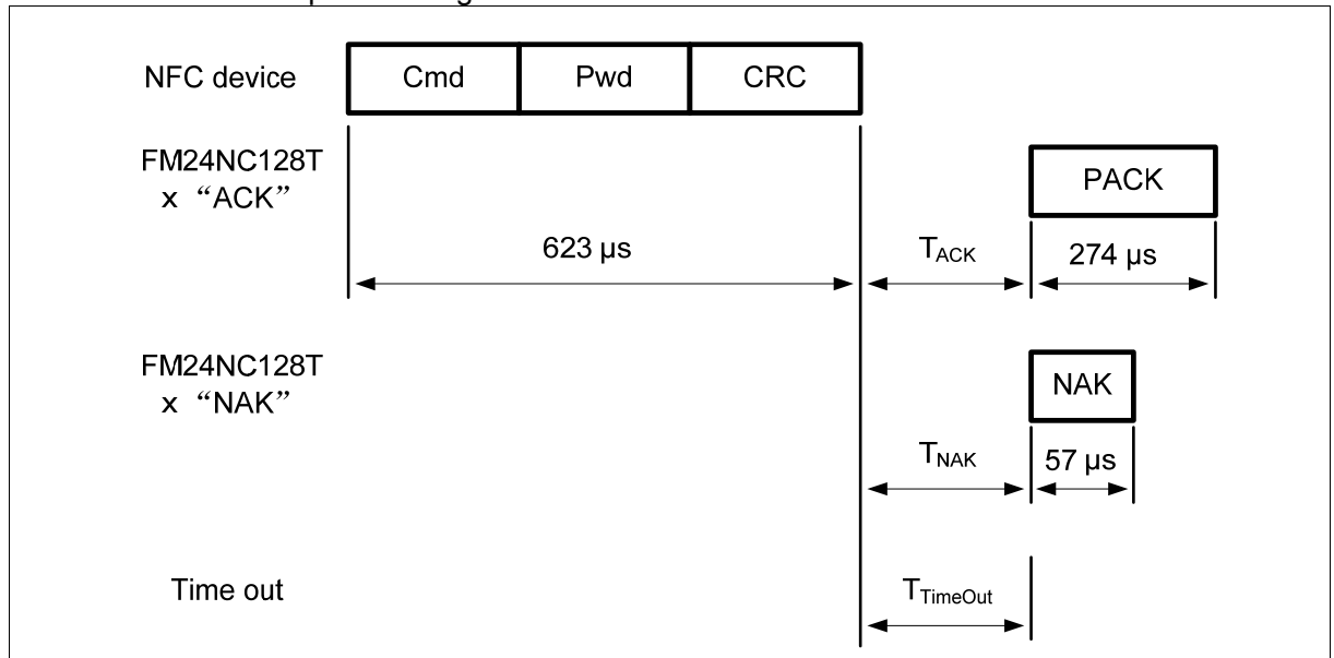
Figure 25 PWD_AUTH command
