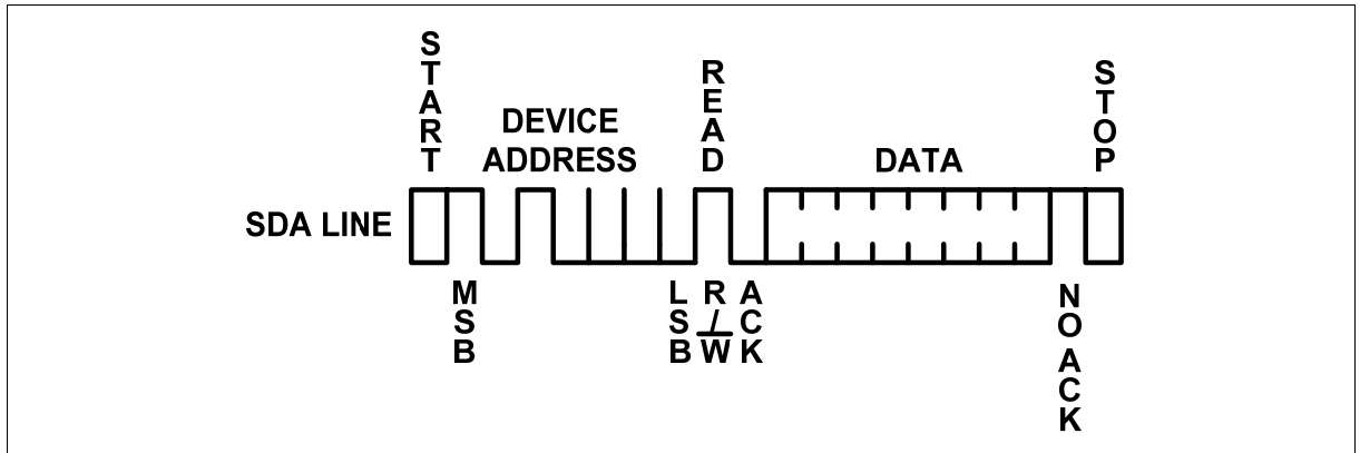
Figure 13 Current address read
