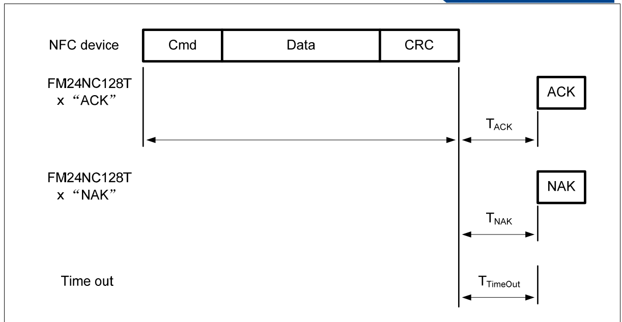
Figure 30 WRITE_RF_DATA_RD_LOCK command
