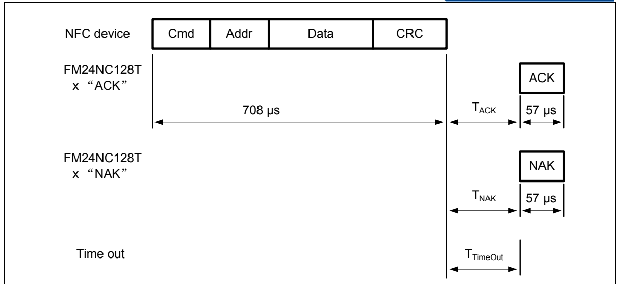
Figure 22 WRITE command
