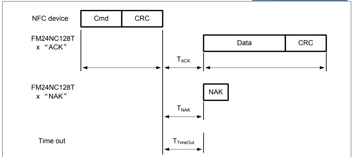
Figure 28 READ_RF_DATA_RD_LOCK command
