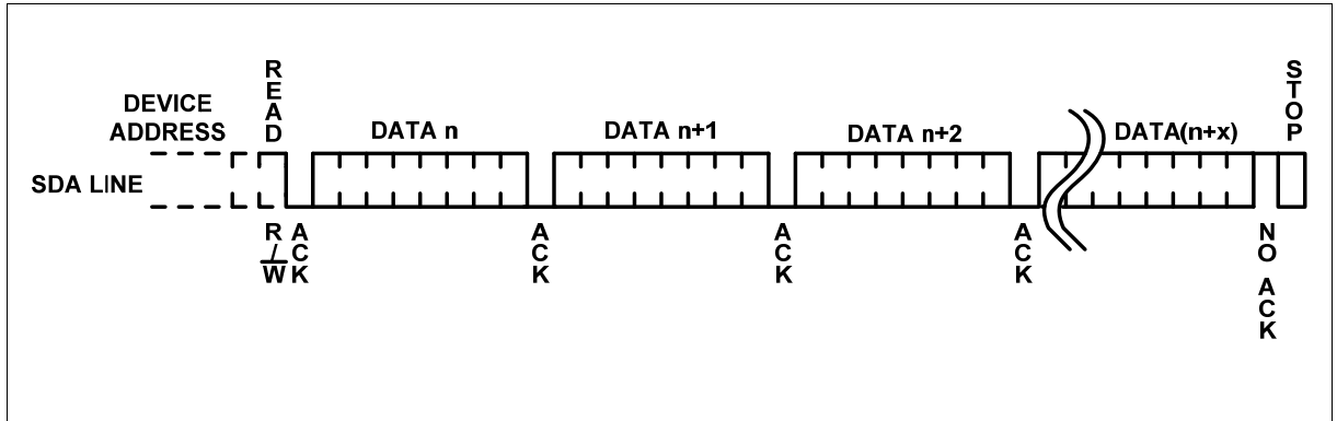
Figure 15 sequential read
