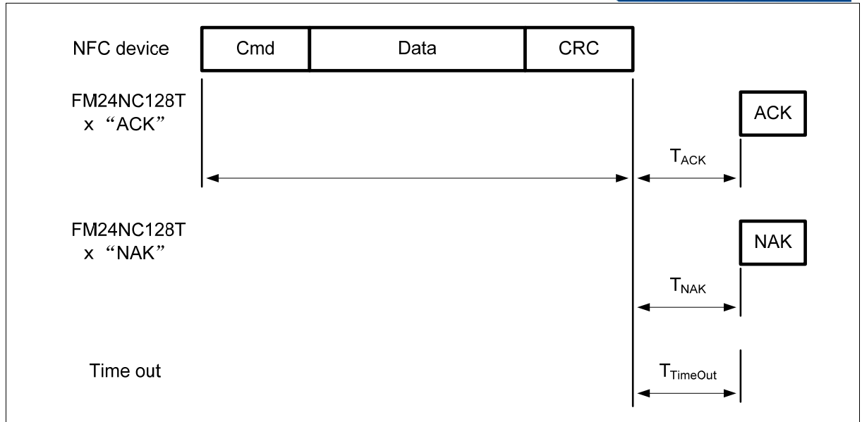
Figure 31 WRITE_RF_DATA_WR_LOCK command
