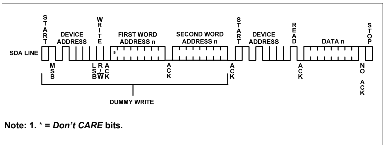
Figure 14 random read
