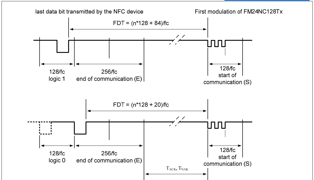
Figure 19 Frame Delay Time (from NFC device to FM24NC128Tx), T_{ACK} and T_{NAK}
