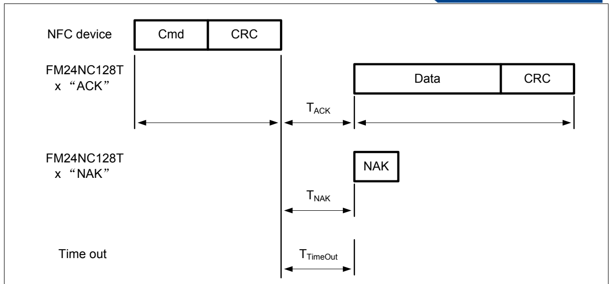
Figure 29 READ_RF_DATA_WR_LOCK command
