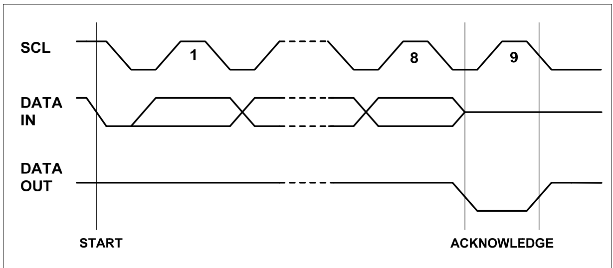
Figure 7 Output Acknowledge
