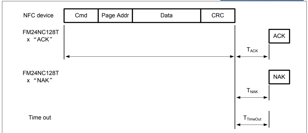
Figure 27 WRITE64B command
