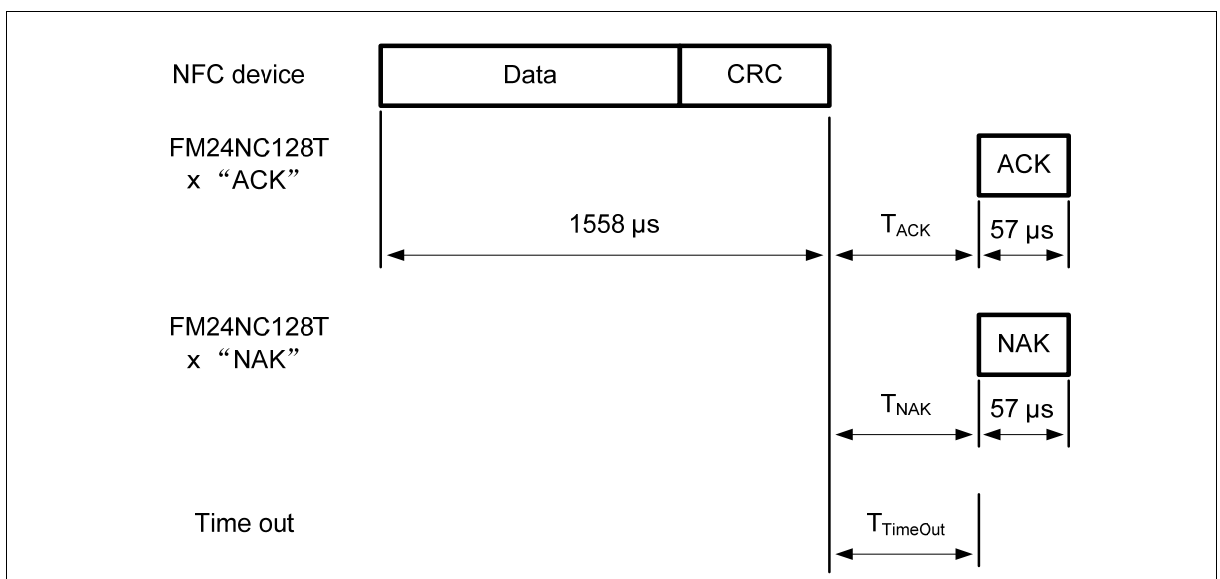
Figure 24 COMPATIBILITY_WRITE command part 2
