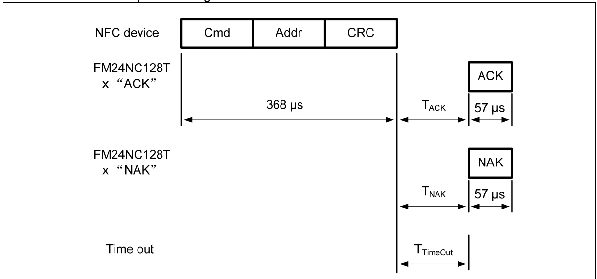
Figure 23 COMPATIBILITY_WRITE command part 1
