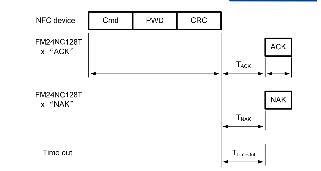
Figure 32 RF_PWD_AUTH command
