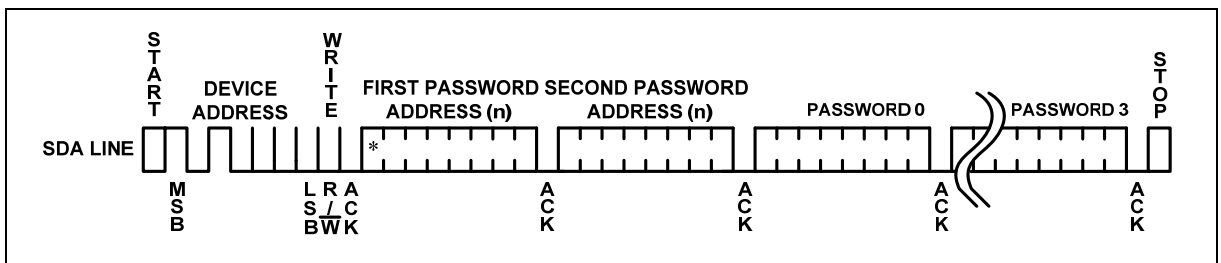
Figure 16 password authentication
