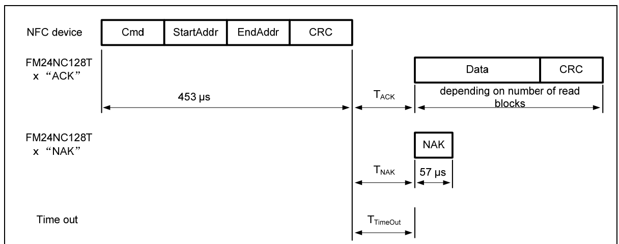
Figure 21 FAST_READ command
