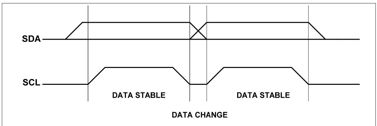
Figure 5 Data Validity
