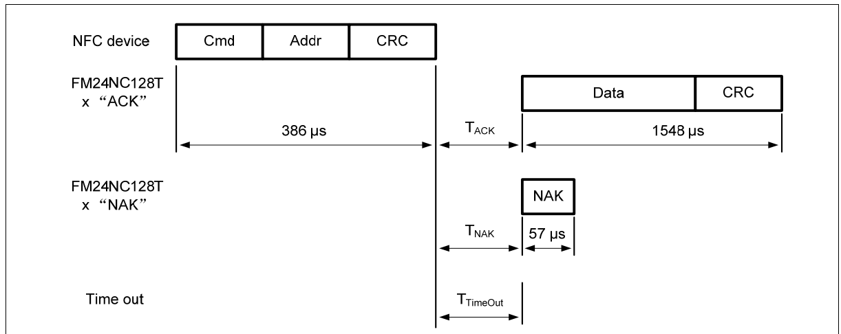
Figure 20 READ command
